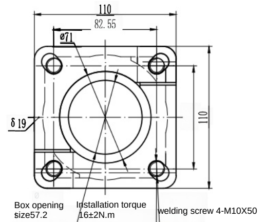
Pressure plate (installation) dimensions
